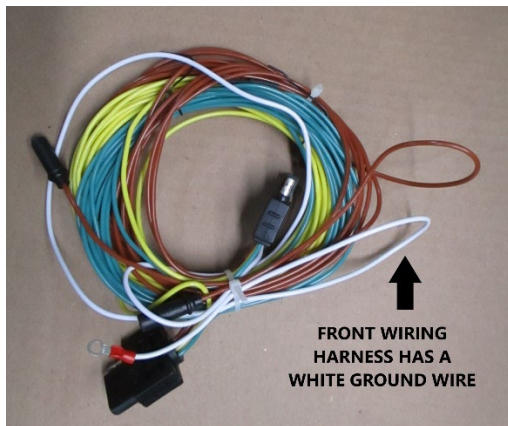
Front Wiring Harness ( Part J )
